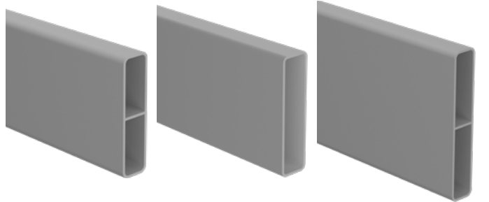
65mm x 16.5mm slat with centre web
